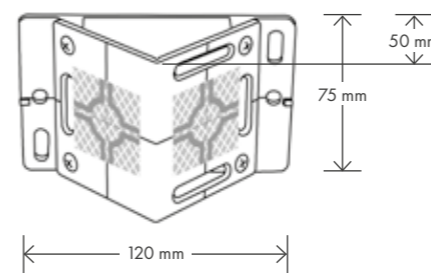
RSAK80 – Carrier Plate with reflective targets 40 x 40 mm
