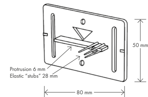
Datum and Axis Markers RS20 and RS21*
