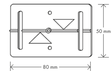
Datum and Axis Markers RS10/RS11*
