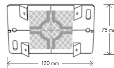
RSAKZ6 – Carrier plate with reflective target 60 x 60 mm
