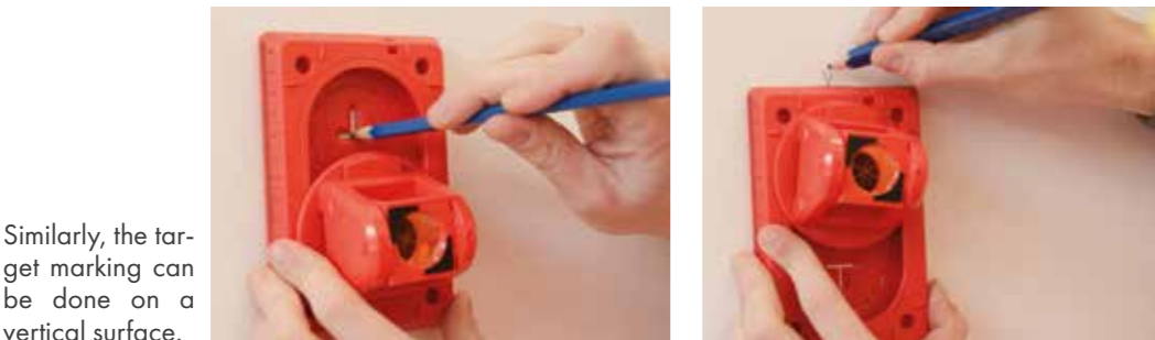
Slide the prism to one side and mark the target position with a pencil.
