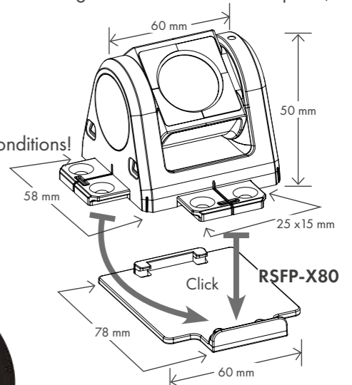
RSMP380 with Ø 25.4 mm mini prism: offset -16.9 (minus 16.9) [Leica +17.5] Tilting axis height RSMP380: 30 mm
