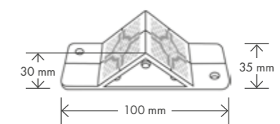
RSAK130 – Plate with angle and 2 reflective targets 30 x 30 mm
